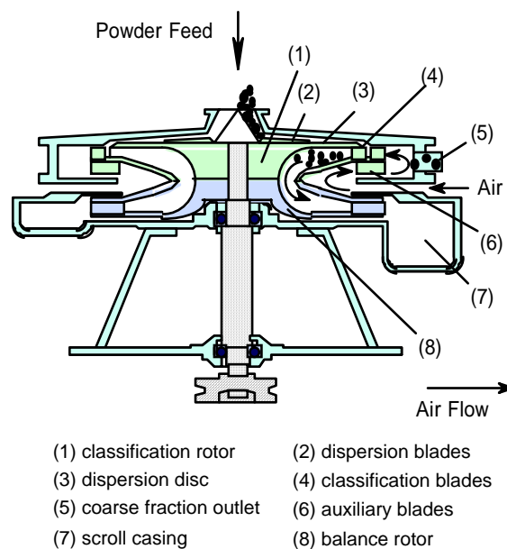
Figure 1 Cross-sectional view of Turbo Classifier
