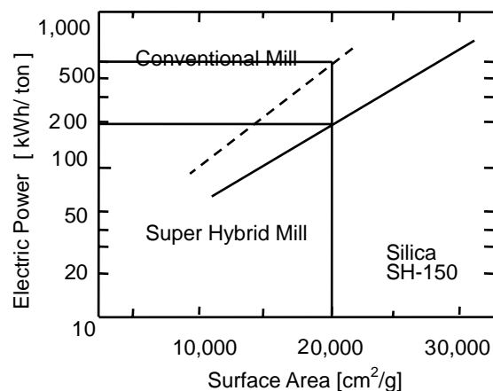
Figure 14 Comparison of electric power usage
