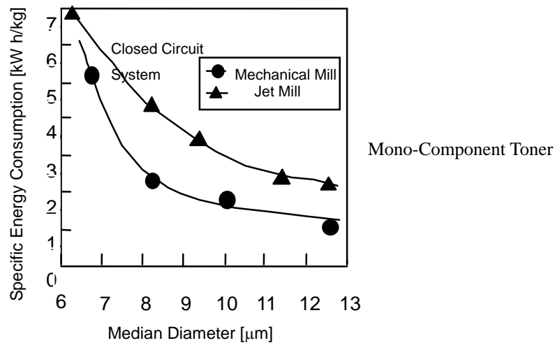
Figure 6 Relationship between the median diameter of product and specific energy consumption of closed circuit grinding system
