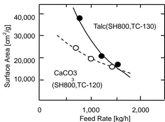
Figure 13 SH-800 Grinding Performance Example
