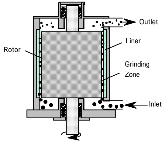
Figure 2 Cross-sectional view of Super Rotor
