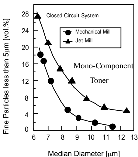
Figure 4 Relation between the median diameter of product and the volume percentage of fine particles less than 5μm
