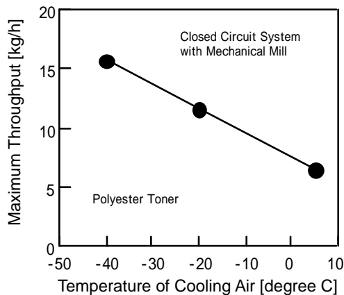
Figure 8 Relation between the temperature of cooling air and the maximum throughput of the mechanical grinding system
