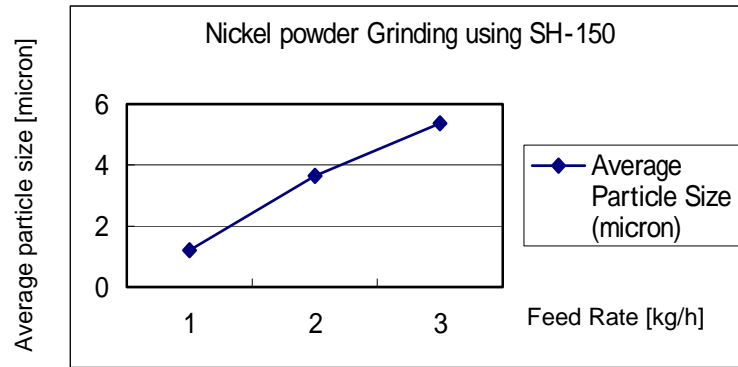
Figure 15 Nickel powder grinding results using SH-150 (TC-25)
