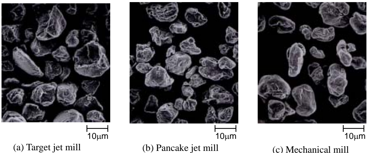
Figure 10 SEM photographs of the toner ground with three kinds of systems
