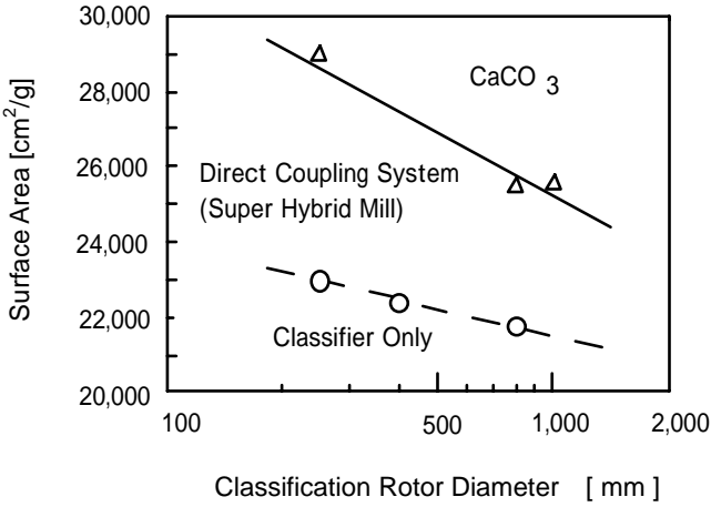
Figure 12 Classification performance improvement by direct coupling
