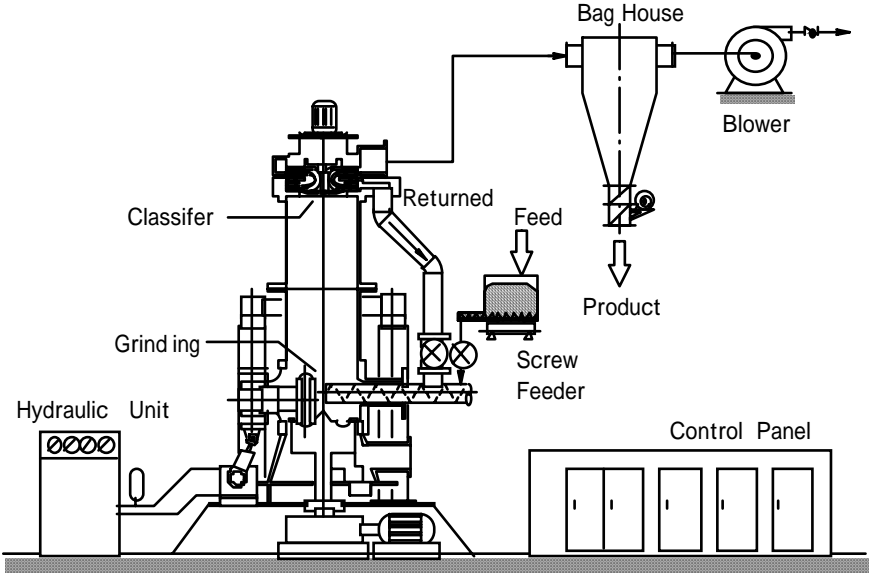
Figure 11 Flow Diagram of Super Hybrid Mill system
